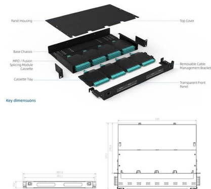
Component Diagram
